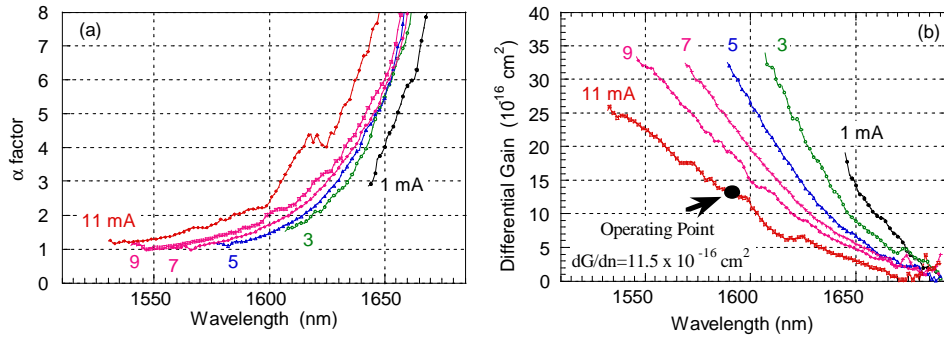
Fig. 7.1. The linewidth enhancement factor (a) and differential gain (b) versus wavelength at various bias currents.
