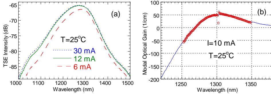
Fig. 2.2. The TSE spectra at 25^{\circ}\text{C} for different currents (a) and modal optical gain spectrum (b) extracted from TSE spectra using the Henry technique (solid line). The gain spectrum extracted from the ASE spectrum taken at the same conditions is also shown (circles).
